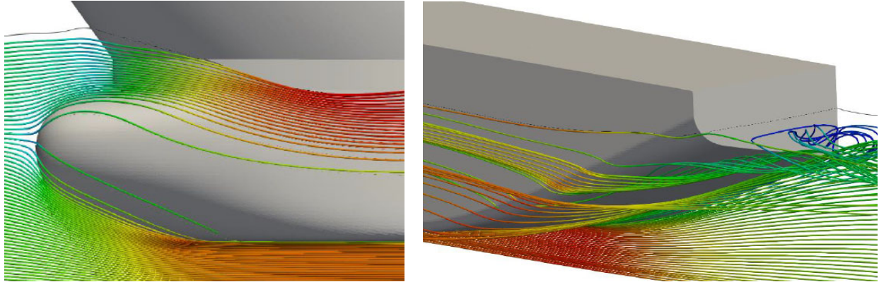
Figure 2: Bow and Stern Streamlines from the CFD Evaluation
