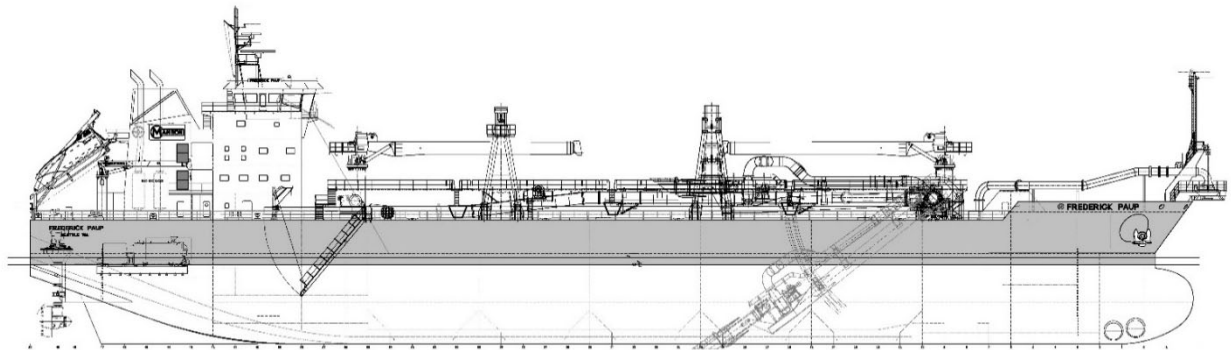
Figure 1: FREDERICK PAUP Outboard Profile
